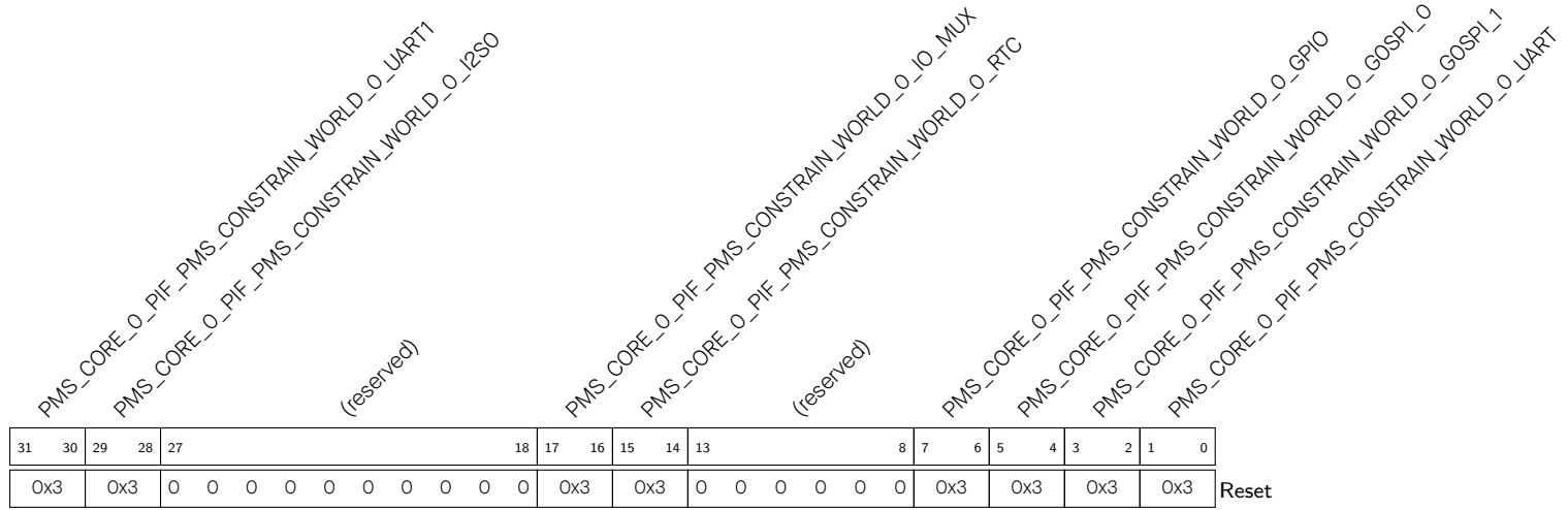
Register 15.50. PMS_CORE_0_PIF_PMS_CONSTRAIN_n_REG (n: 1 - 8) (0x0128 + 4*n)
