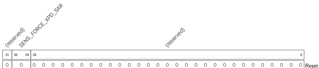
Register 39.18. SENS_SAR_POWER_XPD_SAR_REG (0x003C)
