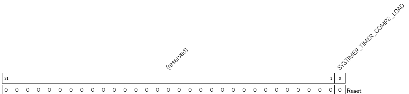
Register 11.25. SYSTIMER_COMP2_LOAD_REG (0x0058)
