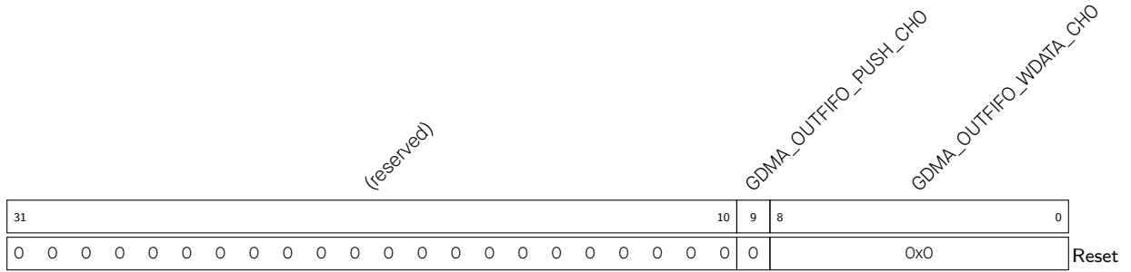
Register 3.7. GDMA_OUT_PUSH_CH n _REG ( n : 0-4) (0x007C+192* n )
