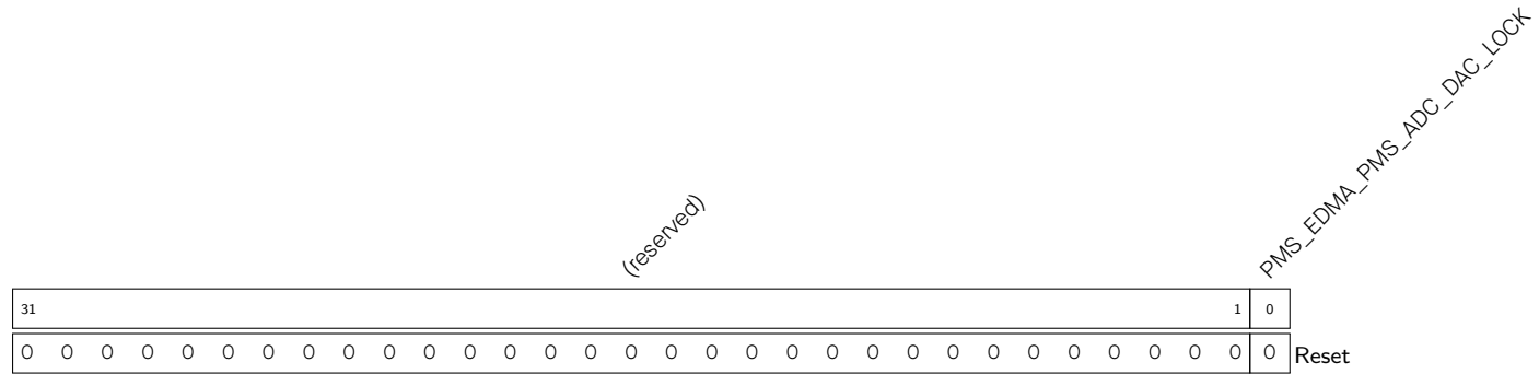
Register 15.88. PMS_EDMA_PMS_ADC_DAC_LOCK_REG (0x02F8)
