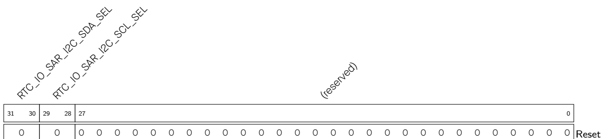
Register 6.57. RTC_IO_SAR_I2C_IO_REG (0x00E4)
