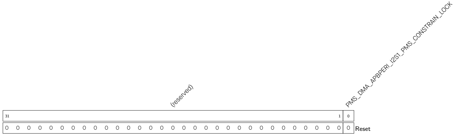
Register 15.14. PMS_DMA_APBPERI_I2S1_PMS_CONSTRAIN_0_REG (0x0058)
