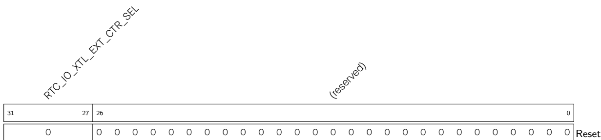
Register 6.56. RTC_IO_XTL_EXT_CTR_REG (0x00E0)
