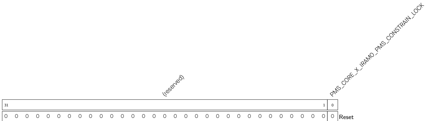
Register 15.40. PMS_CORE_X_IRAMO_PMS_CONSTRAIN_O_REG (0x00D8)
