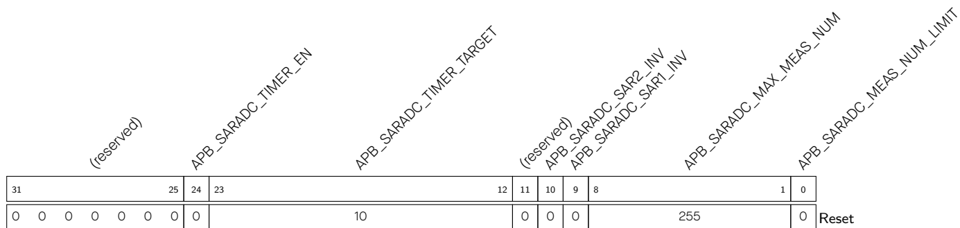
Register 39.57. APB_SARADC_CTRL2_REG (0x0004)
