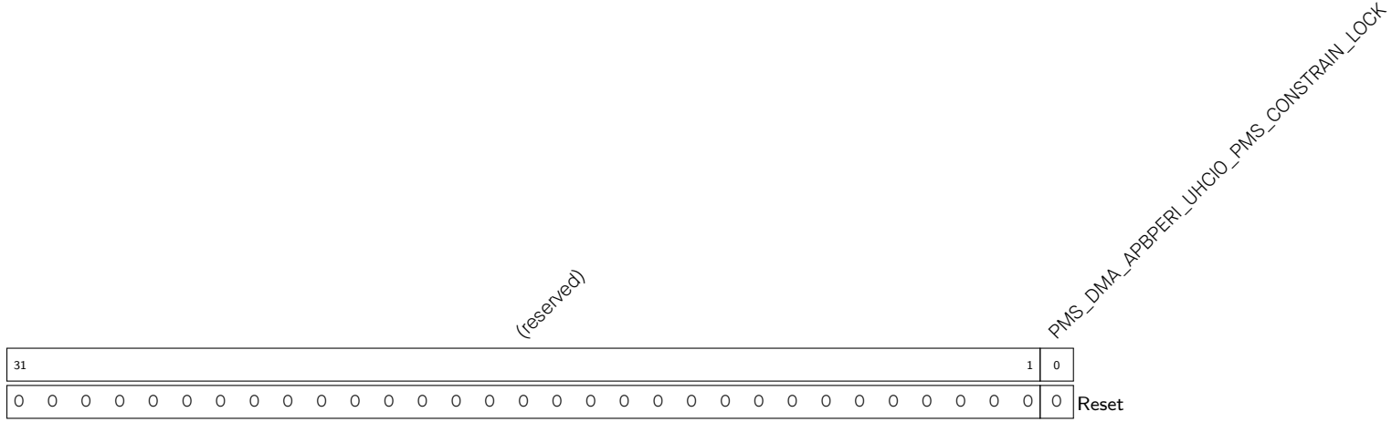
Register 15.10. PMS_DMA_APBPERI_UHCIO_PMS_CONSTRAIN_0_REG (0x0048)
