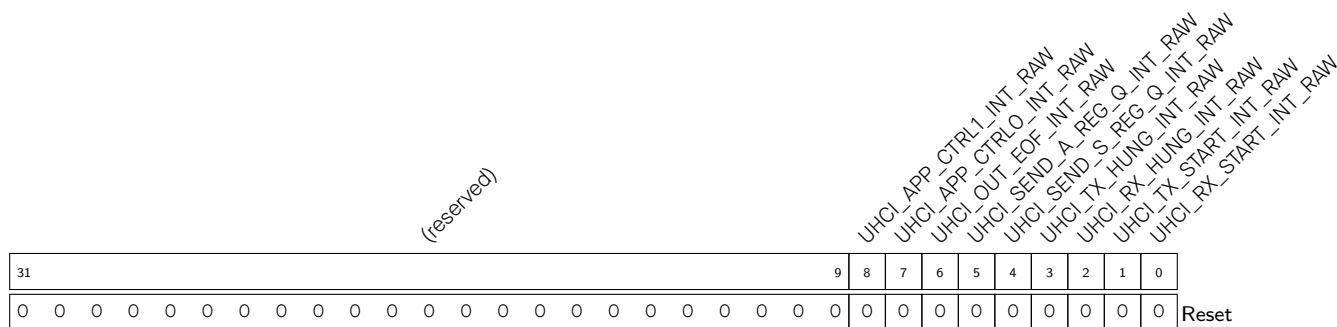
Register 26.59. UHCI_INT_RAW_REG (0x0004)
