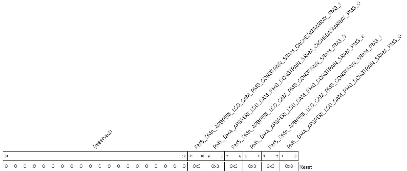
Register 15.25. PMS_DMA_APBPERI_LCD_CAM_PMS_CONSTRIN_1_REG (0x0094)
