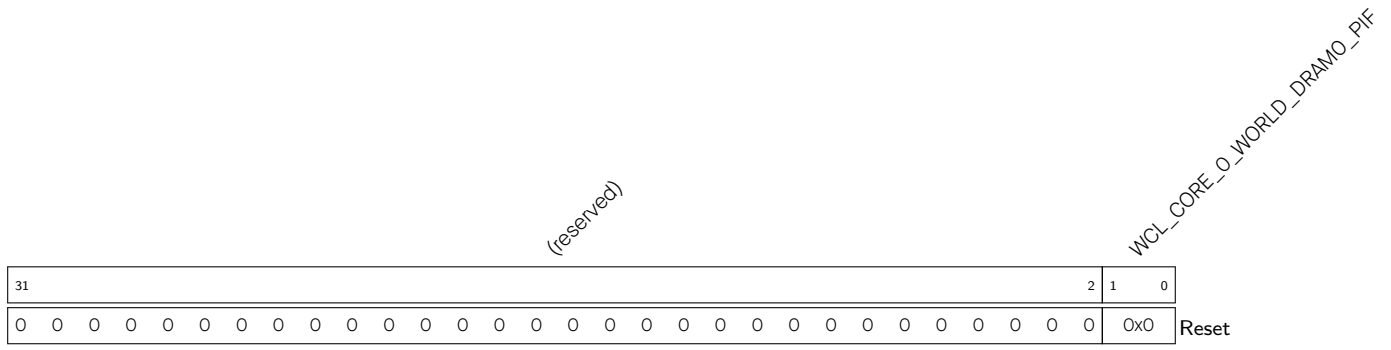
Register 16.13. WCL_CORE_O_World_DRam0_PIF_REG (0x0154)
