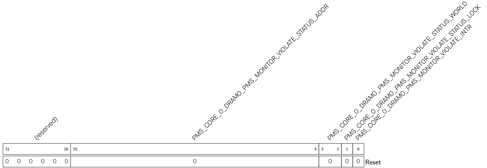
Register 15.94. PMS_CORE_0_DRAMO_PMS_MONITOR_2_REG (0x010C)
