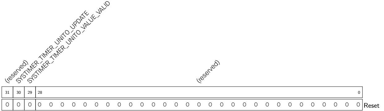
Register 11.2. SYSTIMER_UNIT0_OP_REG (0x0004)
