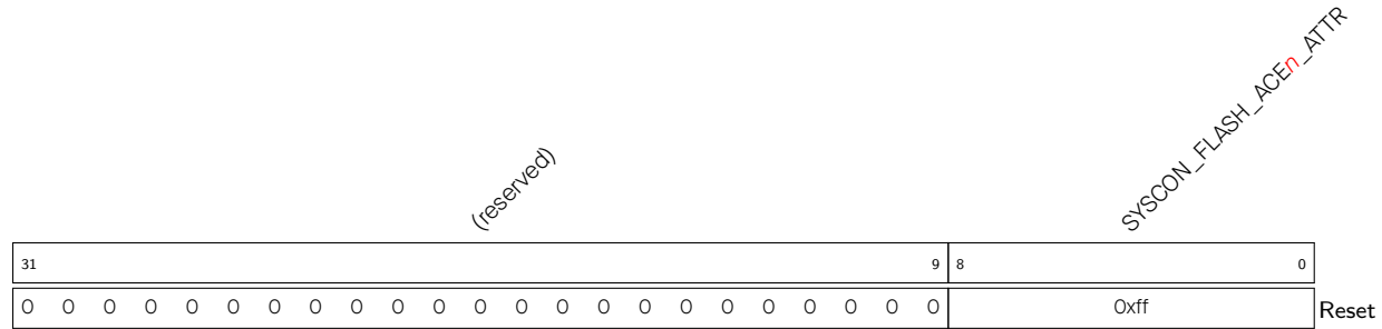
Register 15.102. SYSCON_FLASH_ACEN_ATTR_REG ( n: 0 - 3 ) (0x0028 + 4*n)
