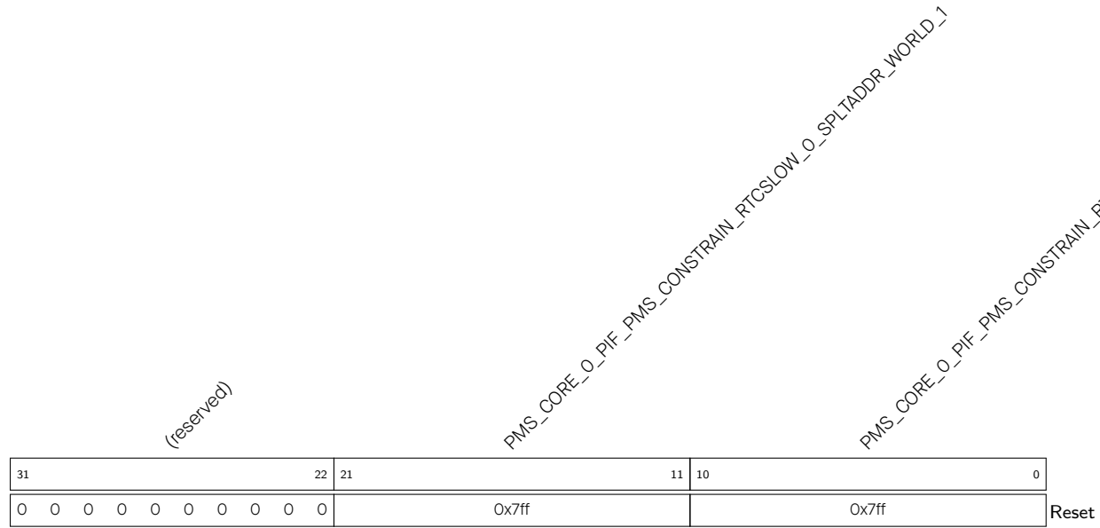
Register 15.53. PMS_CORE_0_PIF_PMS_CONSTRIN_11_REG (0x0150)
