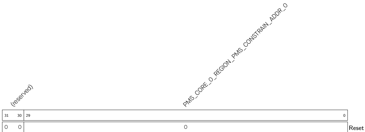
Register 15.60. PMS_CORE_0_REGION_PMS_CONSTRAIN_n_REG (n: 3 - 14) (0x016C + 4*n)
