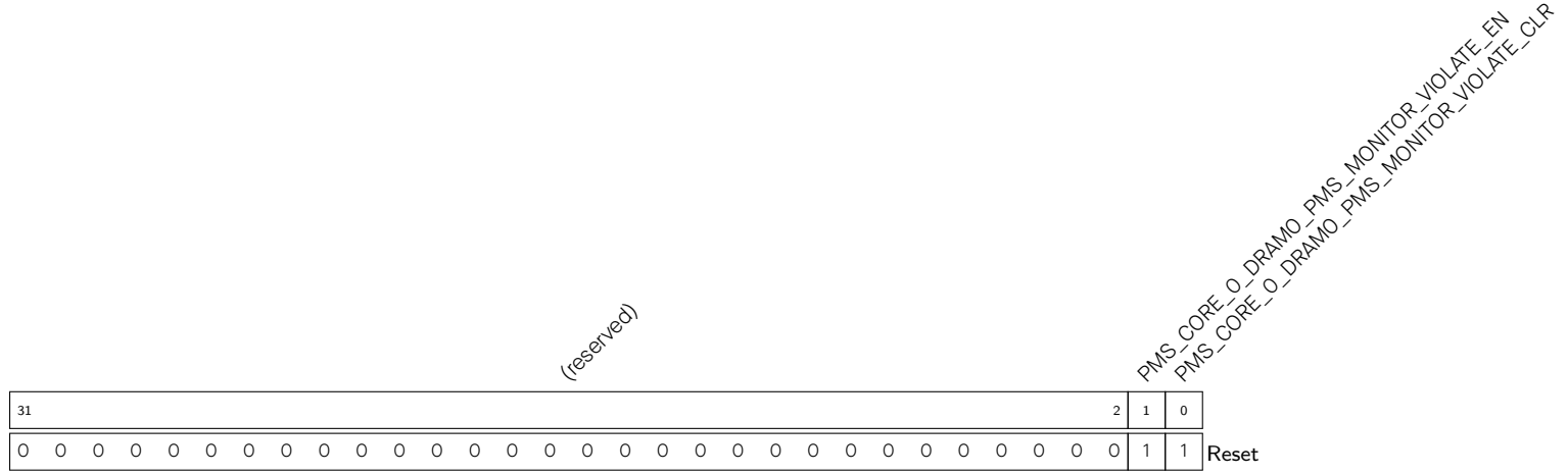
Register 15.48. PMS_CORE_0_DRAMO_PMS_MONITOR_1_REG (0x0108)
