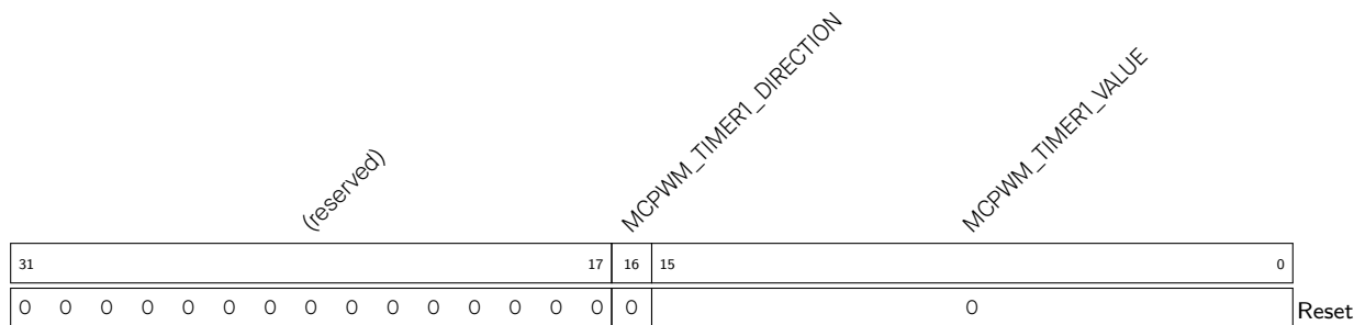
Register 36.9. MCPWM_TIMER1_STATUS_REG (0x0020)
