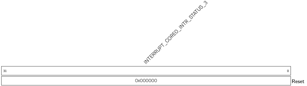
Register 9.88. INTERRUPT_CORE0_INTR_STATUS_3_REG (0x0198)
