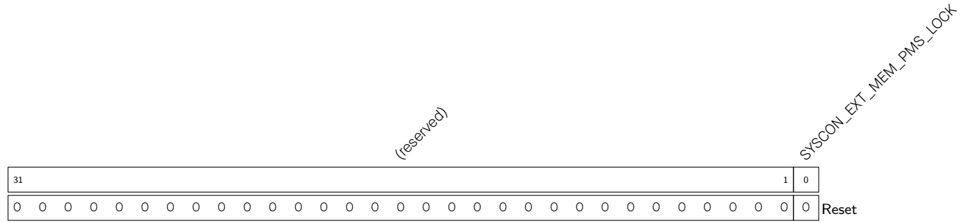
Register 15.101. SYSCON_EXT_MEM_PMS_LOCK_REG (0x0020)
