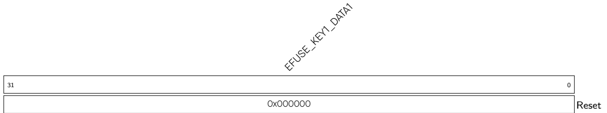
Register 5.49. EFUSE_RD_KEY1_DATA1_REG (0x00C0)
