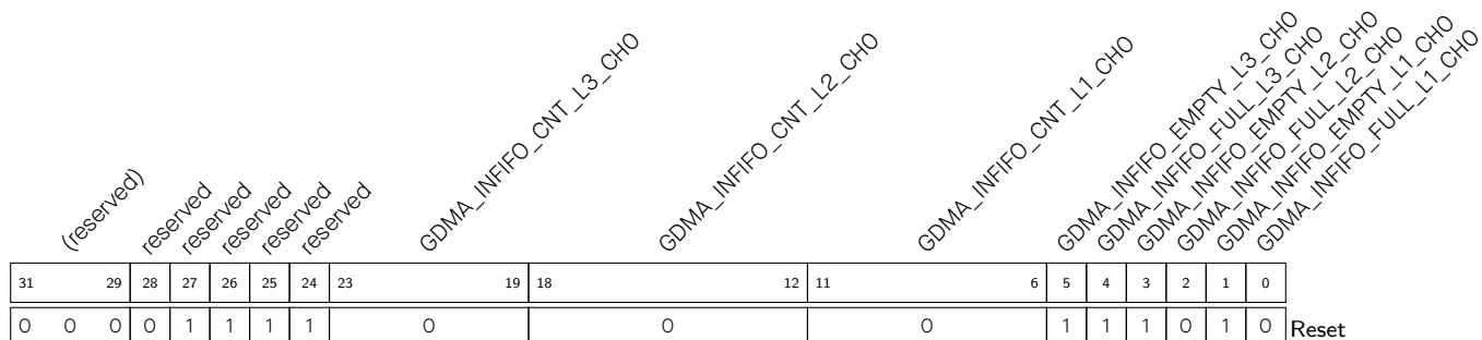
Register 3.23. GDMA_INFIFO_STATUS_CH n _REG ( n : 0-4) (0x0018+192* n )
