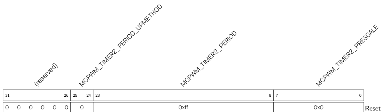
Register 36.10. MCPWM_TIMER2_CFG0_REG (0x0024)
