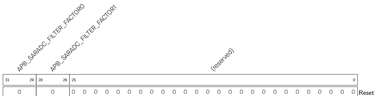
Register 39.58. APB_SARADC_FILTER_CTRL1_REG (0x0008)
