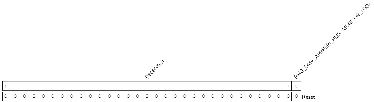
Register 15.30. PMS_DMA_APBPERI_PMS_MONITOR_0_REG (0x00B0)
