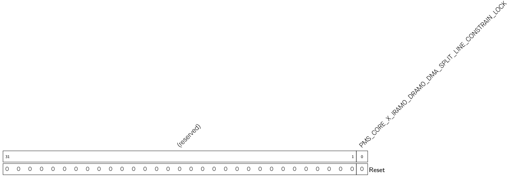
Register 15.34. PMS_CORE_X_IRAMO_DRAMO_DMA_SPLIT_LINE_CONSTRAIN_O_REG (0x00C0)
