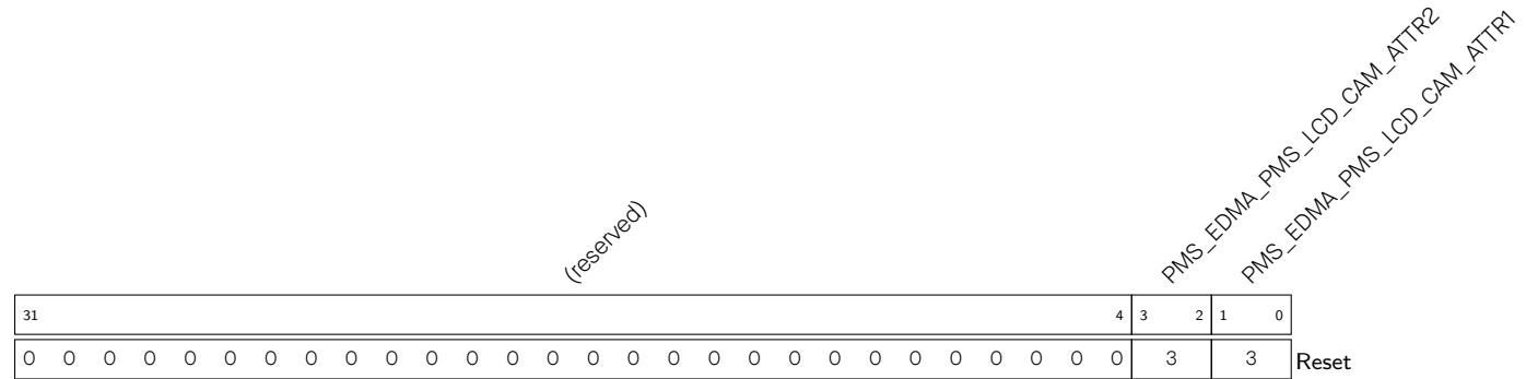
Register 15.83. PMS_EDMA_PMS_LCD_CAM_REG (0x02E4)
