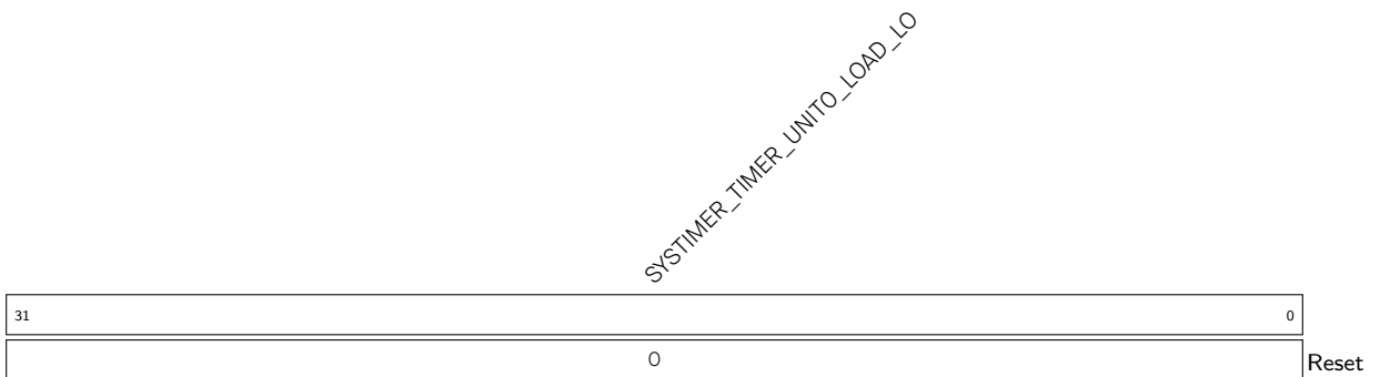
Register 11.4. SYSTIMER_UNIT0_LOAD_LO_REG (0x0010)
