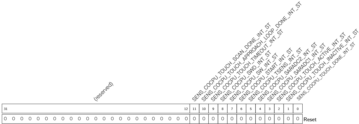
Register 2.7. SENS_SAR_COCPU_INT_ST_REG (0x00F0)
