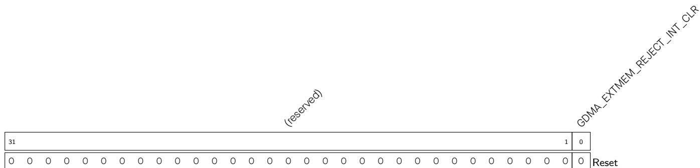
Register 3.22. GDMA_EXTMEM_REJECT_INT_CLR_REG (0x0408)
