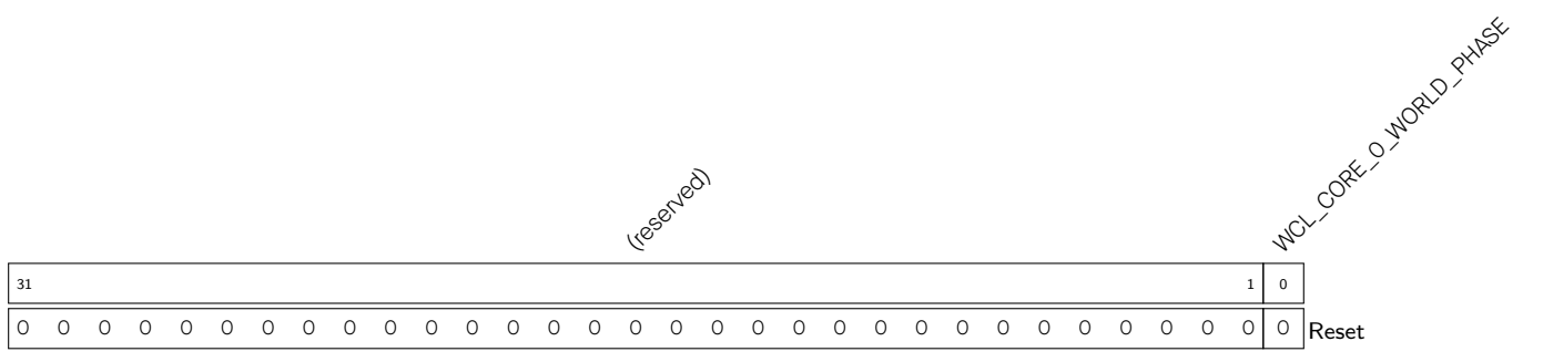
Register 16.14. WCL_CORE_O_World_Phase_REG (0x0158)
