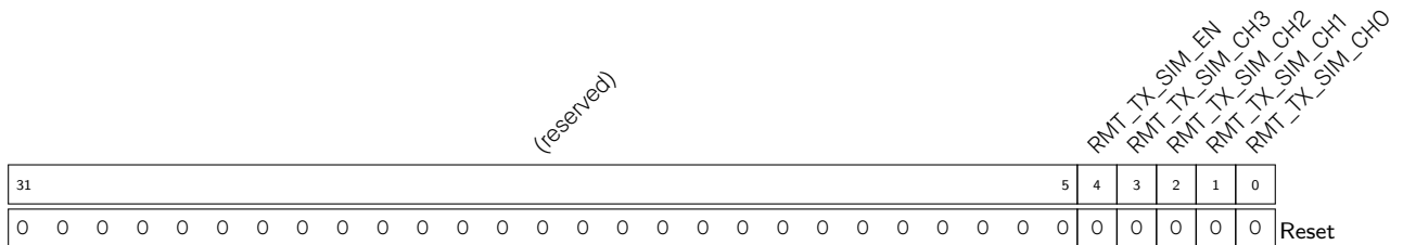
Register 3717. RMT_TX_SIM_REG (0x00C4)
