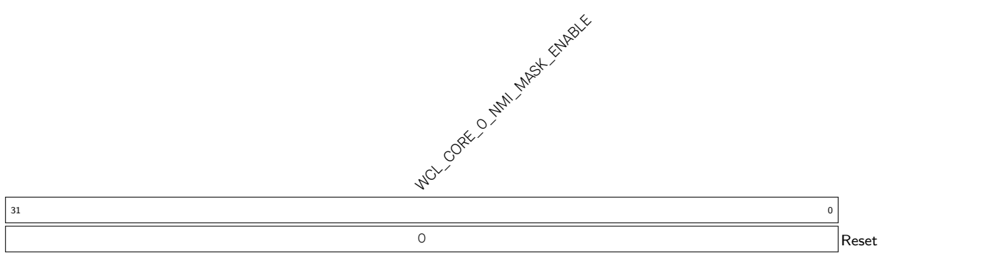
Register 16.15. WCL_CORE_O_NMI_MASK_ENABLE_REG (0x0180)
