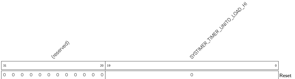
Register 11.3. SYSTIMER_UNIT0_LOAD_HI_REG (0x000C)
