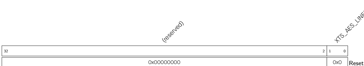
Register 24.2. XTS_AES_LINESIZE_REG (0x0340)
