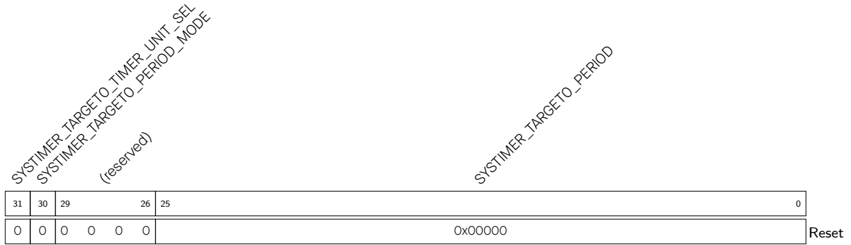
Register 12.16. SYSTIMER_TARGET0_CONF_REG (0x0034)
