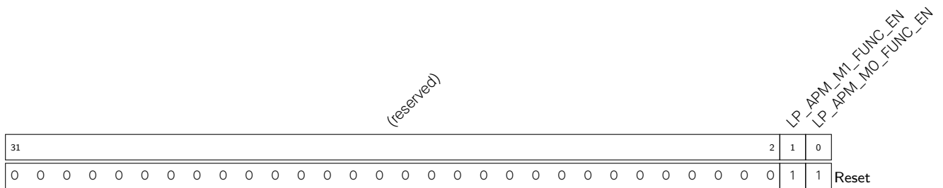
Register 15.29. LP_APM_FUNC_CTRL_REG (0x00C4)
