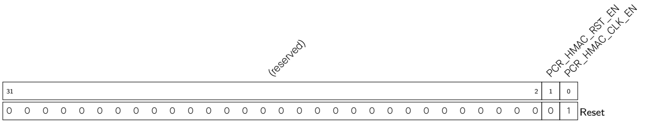
Register 8.54. PCR_HMAC_CONF_REG (0x00E4)
