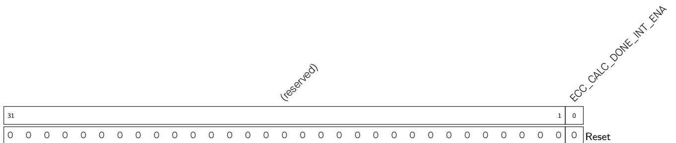
Register 19.3. ECC_MULT_INT_ENA_REG (0x0014)
