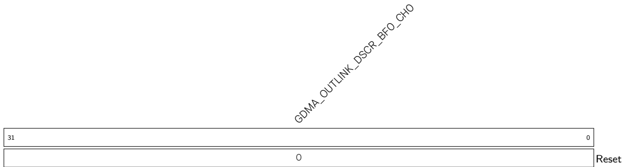
Register 4.32. GDMA_OUT_DSCR_BFO_CH n _REG ( n : 0-2) (0x00F4+0xC0* n )
