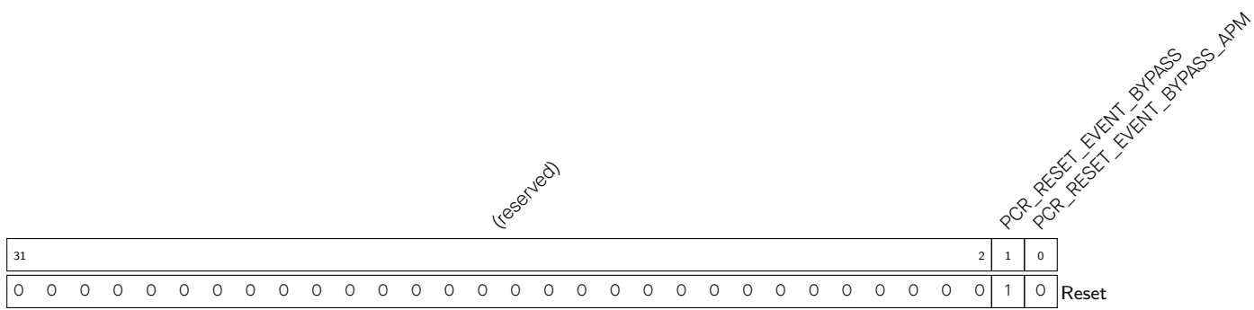
Register 8.72. PCR_RESET_EVENT_BYPASS_REG (0x0FF0)
