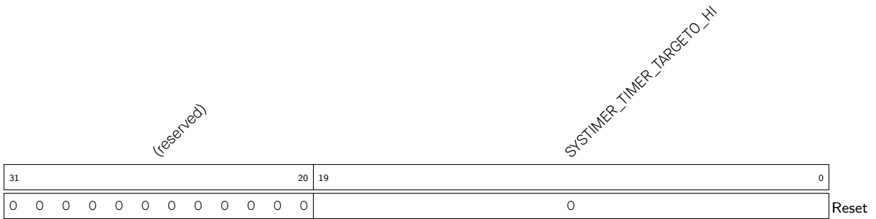
Register 12.14. SYSTIMER_TARGETO_HI_REG (0x001C)
