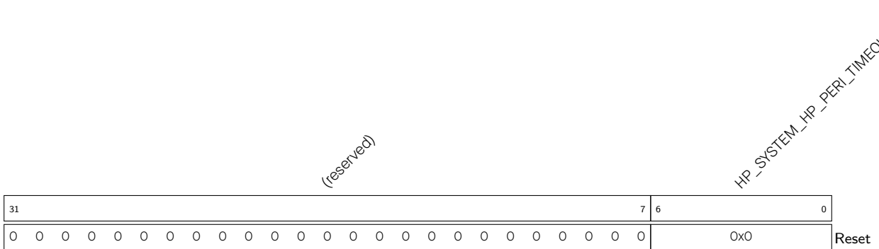
Register 16.9. HP_SYSTEM_HP_PERI_TIMEOUT_UID_REG (0x0020)
