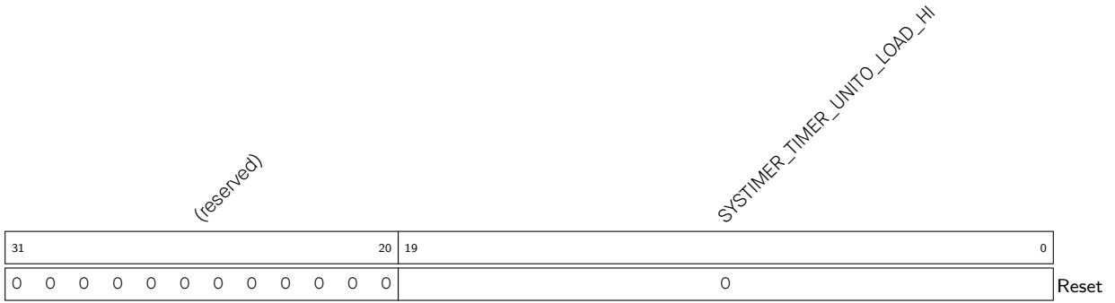
Register 12.3. SYSTIMER_UNIT0_LOAD_HI_REG (0x000C)
