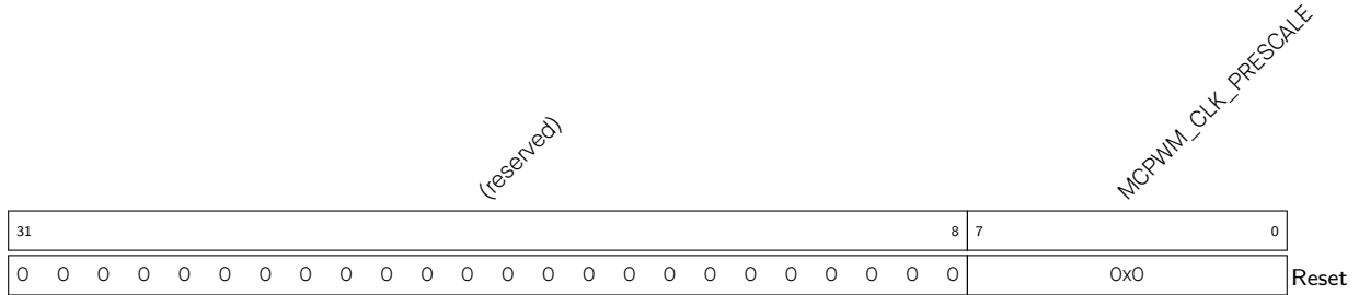
Register 35.1. MCPWM_CLK_CFG_REG (0x0000)
