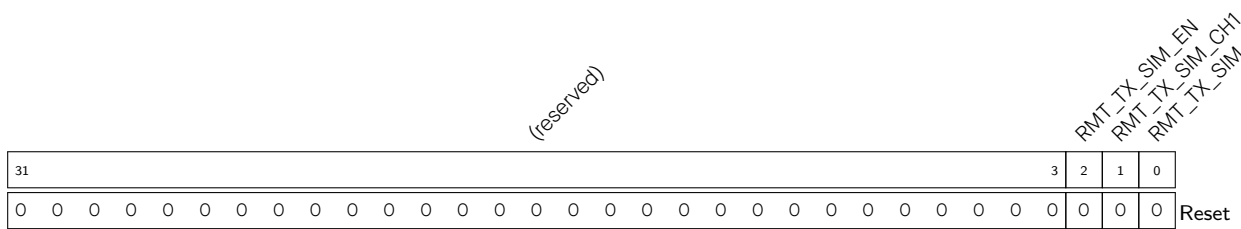
Register 36.16. RMT_TX_SIM_REG (0x006C)
