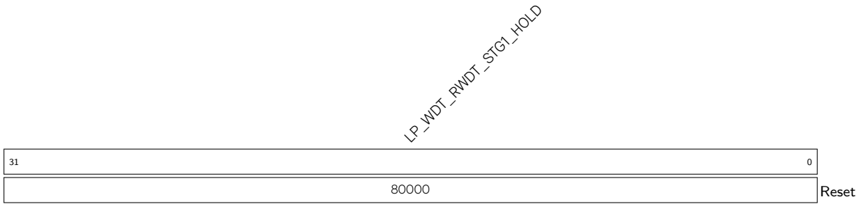
Register 14.3. LP_WDT_RWDT_CONFIG2_REG (0x0008)
