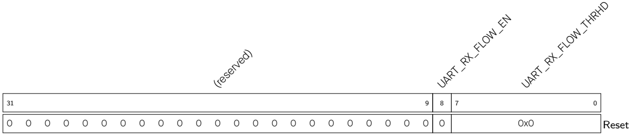
Register 26.11. UART_HWFC_CONF_SYNC_REG (0x002C)
