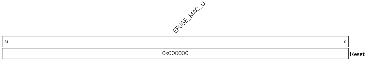
Register 6.18. EFUSE_RD_MAC_SPI_SYS_0_REG (0x0044)
