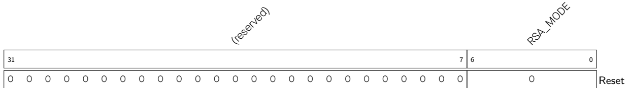
Register 21.2. RSA_MODE_REG (0x0804)
