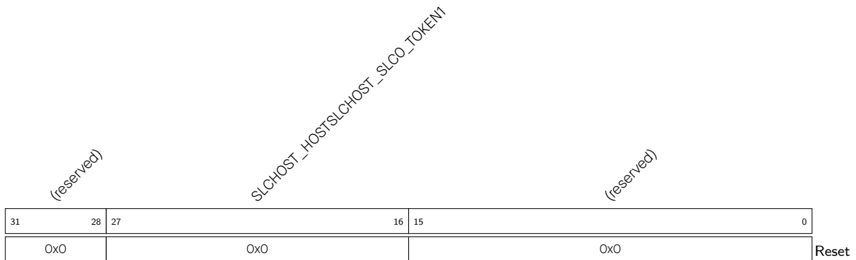
Register 33.50. SLCHOST_SLC0HOST_TOKEN_RDATA_REG (0x0044)
