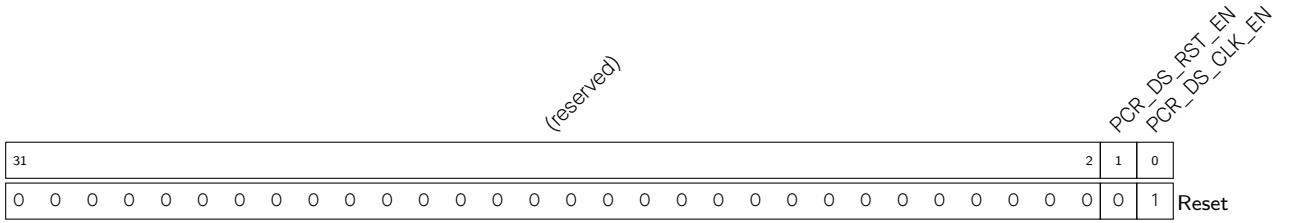
Register 8.53. PCR_DS_CONF_REG (0x00E0)
