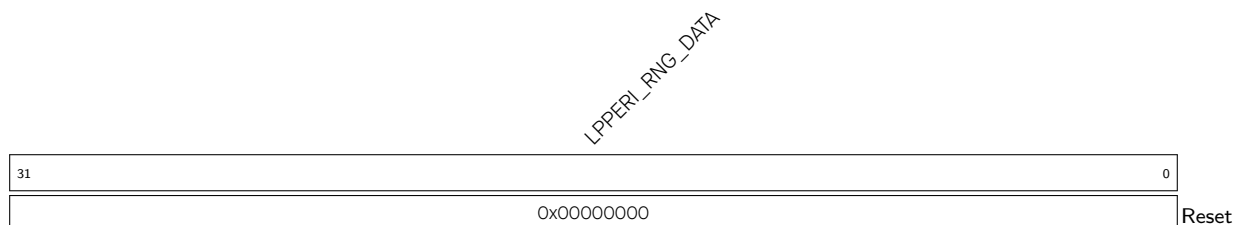
Register 25.1. LPPERI_RNG_DATA_REG (0x600B_2808)
