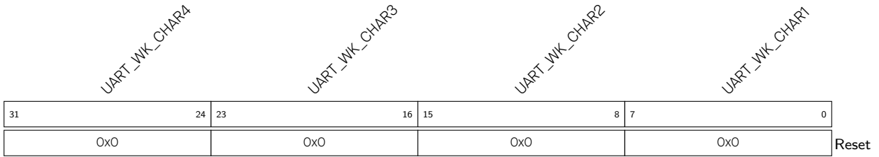
Register 26.12. UART_SLEEP_CONFO_REG (0x0030)
