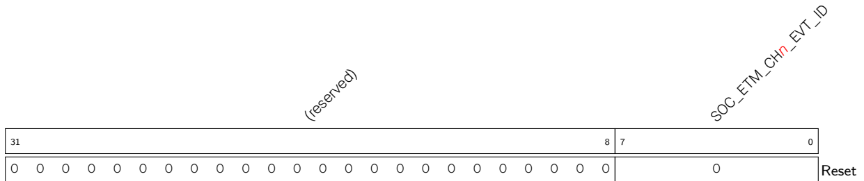
Register 11.7. SOC_ETM_CH n _EVT_ID_REG ( n : 0-49) (0x0018+0x8* n )
